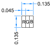
DETAIL A SCALE 60:1
